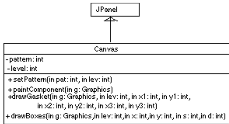
Figure 12.32: Design of a drawing Canvas class.
