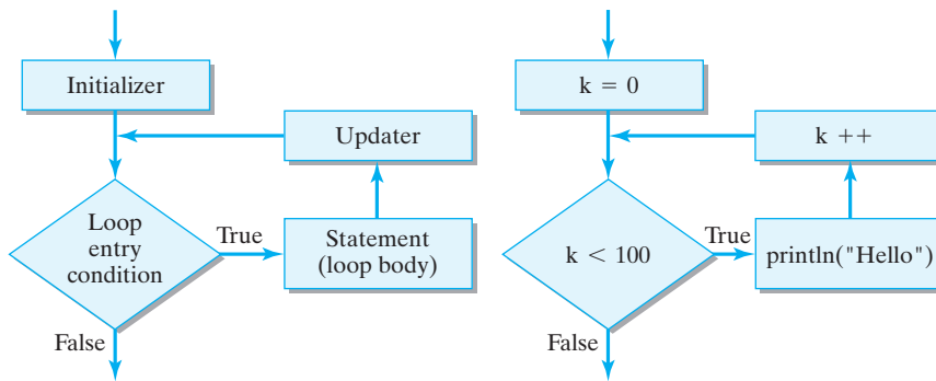
Figure 6.1: Flowchart of the for statement.
