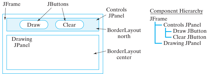
Figure 14.8: GUI design for the dot-drawing program.
