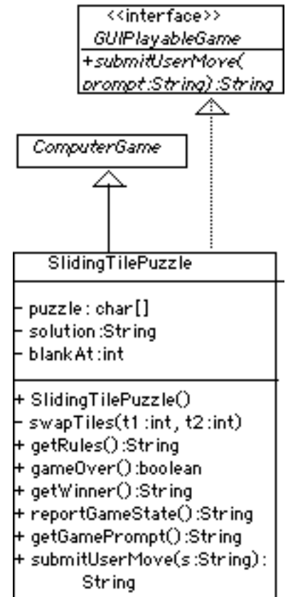
FIGURE 9.37 The SlidingTilePuzzle is a ComputerGame that implements the GUIPlayableGame interface.
