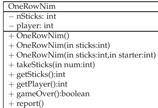
Figure 3.5: A UML class diagram for the expanded OneRowNim .
