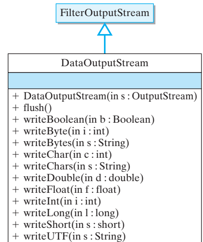
FIGURE 11.18 The java.io.DataOutputStream class contains methods for writing all types of data.
