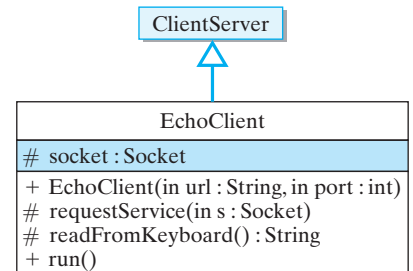
FIGURE 15.29 Design of the EchoClient class.
