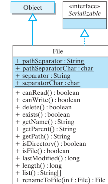
FIGURE 11.16 The java.io.File class.
