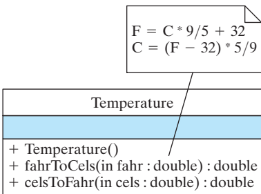
FIGURE 5.4 The Temperature class. Note that static elements are underlined in UML. (NEEDS REVISION)
