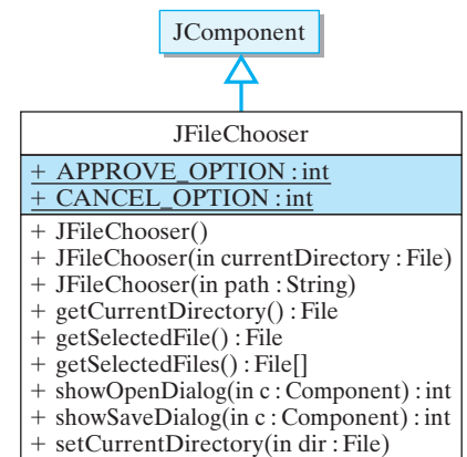
FIGURE 11.29 The javax.swing.JFileChooser class.
