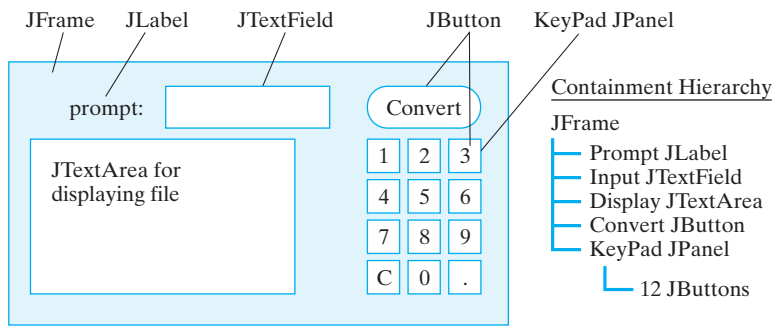
Figure 13.14: A widget hierarchy showing the containment relationships among the components.
