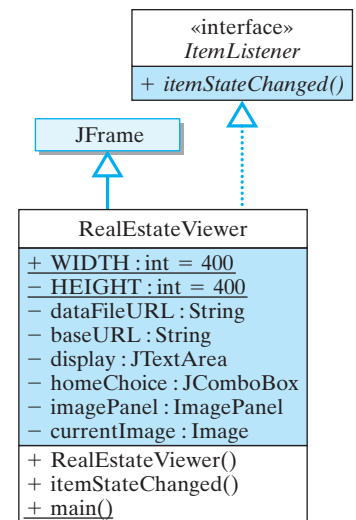
FIGURE 15.16 The RealEstateViewer class defines the user interface.
