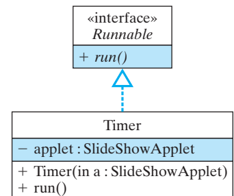
FIGURE 15.11 The Timer class delays the applet thread between each slide.
